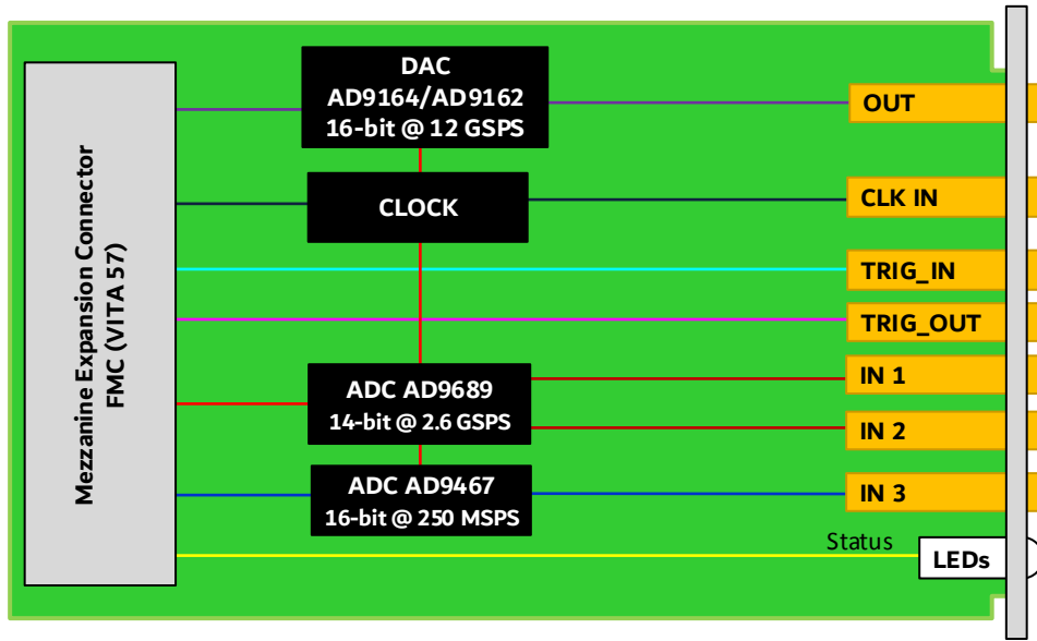
Figure 2: FMC251 Functional Block Diagram
